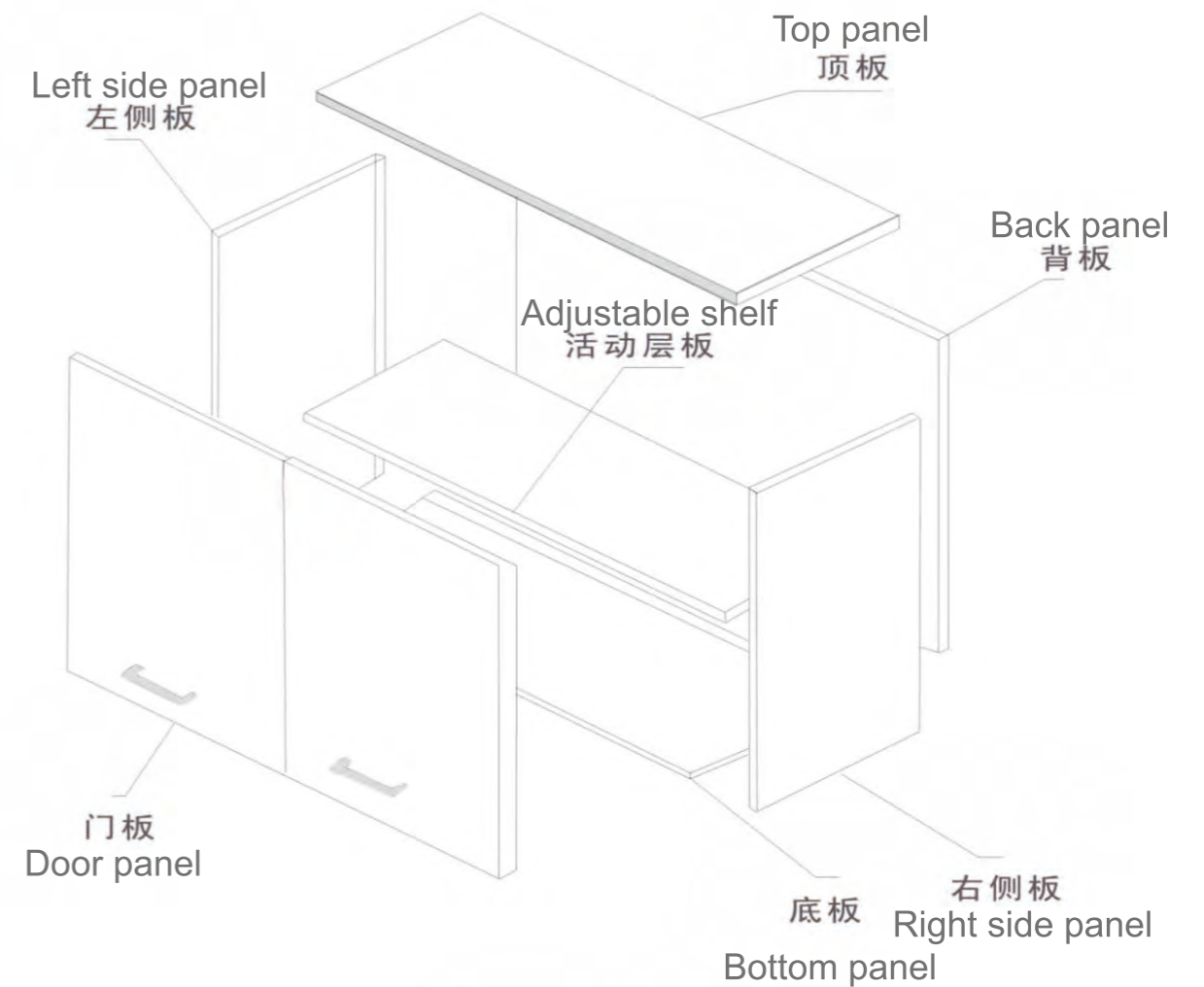
吊 柜 Wall cabinet
